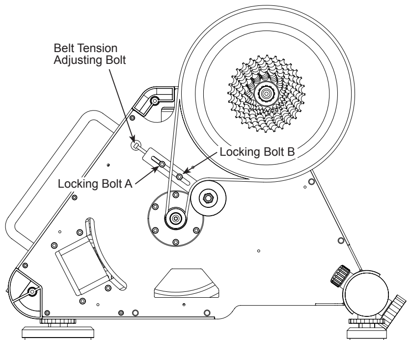
(inside mechanism after removing the side cover)
